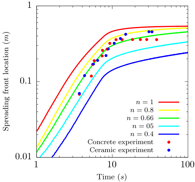
Fig. 9. Simulated front progress for Arr = 7.10^{-3} , \tau_y = 100 Pa and different values of the fluid index n , and experimental results for the VEU7 test, for both concrete and ceramic substrate channels. log-log representation of Fig. 8.
