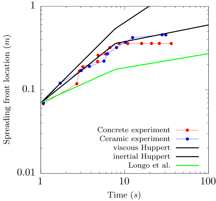
Fig. 6. Experimental front position evolution and its comparison to self-similar solutions from Huppert (1982), Longo et al. (2015) for various geometries. We assume from this comparison that the process of corium spreading is mainly viscous during corium inlet feeding.
