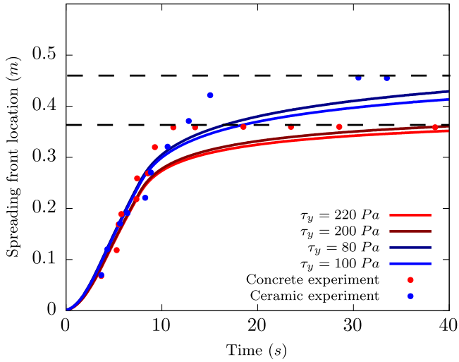
Fig. 10. Simulated front progress for n = 0.66 , Arr = 7.10^{-3} and different values of the initial yield stress \tau_y , and experimental results for the VEU7 test, for both concrete and ceramic substrate channels.
