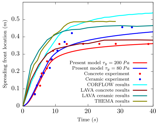
Fig. 15. Comparison between the LAVA, CORFLOW, THEMA codes and the present model.
