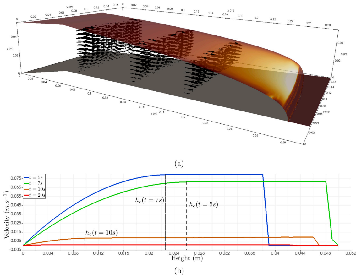
Fig. 12. (a) Tridimensional reconstruction of the velocity. The top surface color represents height-averaged temperature. (b) Velocity profiles along the z -axis at t = 5 s (during melt supplying), t = 7 s (close to the end of melt supplying), t = 10 s (after the end of melt supply, toward melt front stop) and t = 20 s at x = 12 cm and y = 10 cm.
