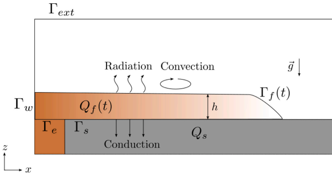
Fig. 2. Corium spreading: its geometry and notations.
