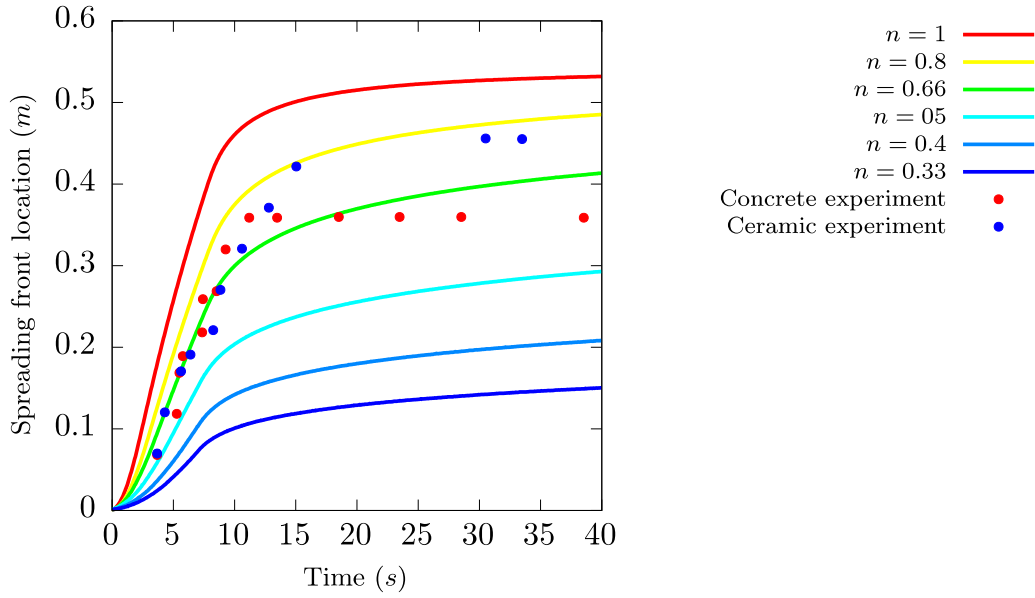
Fig. 8. Simulated front progress for Arr = 7.10^{-3} , \tau_y = 100 Pa and different values of the fluid index n , and experimental results for the VEU7 test, for both concrete and ceramic substrate channels.
