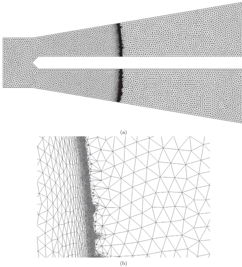
Fig. 3. (a) Auto-generated mesh and (b) Zoom of mesh (a) at the front of the spread.
