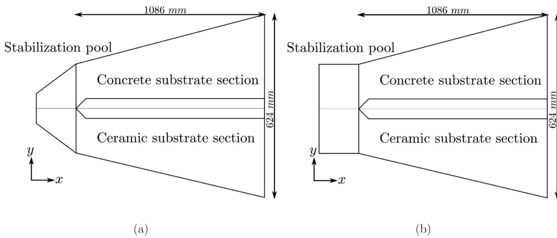
Fig. 5. (a) VEU7 spreading test diagram and (b) geometry used for simulations.
