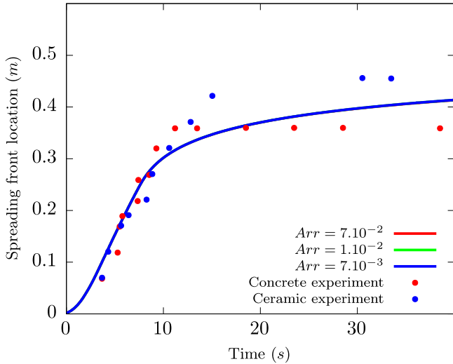
Fig. 7. Simulated front progress for n = 1 , \tau_y = 100 Pa and different values of the Shaw model coefficient Arr , and experimental results for the VEU7 test, for both concrete and ceramic substrate channels.
