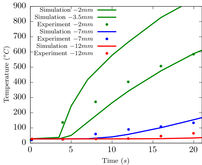
Fig. 13. Concrete substrate temperature evolution for the VEU7 experiment and its simulation, for thermocouples at x = 12 cm, y = 10 cm and z = -2, -7, -12 mm.
