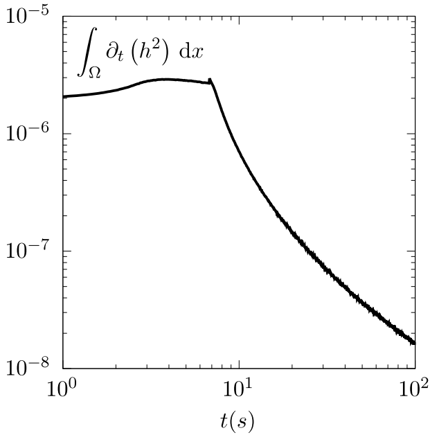
Fig. 11. Evolution of \int_{\Omega} \partial_t (h^2) dx , for the simulation with n = 0.66 and \tau_y = 200 Pa. It shows that the movement of the melt slows down quickly once corium source stops at t = 7.7 s.
