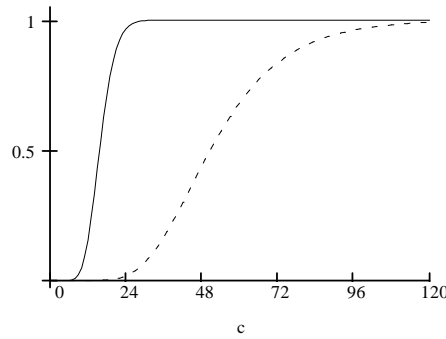
Fig. 2: Limiting probability distribution of the events E_d (solid) and S_d (dots) for d = 4 , with respect to the expected cardinality c of the random class. Inflection points at c = 15 and c = 44 , respectively.
